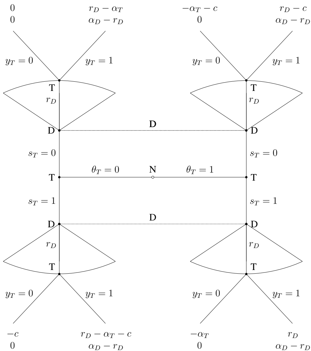
Figure 1: Game Tree
